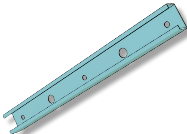
Figure 06 – Isometric view of typical 25/14 wall-tie retention channel
